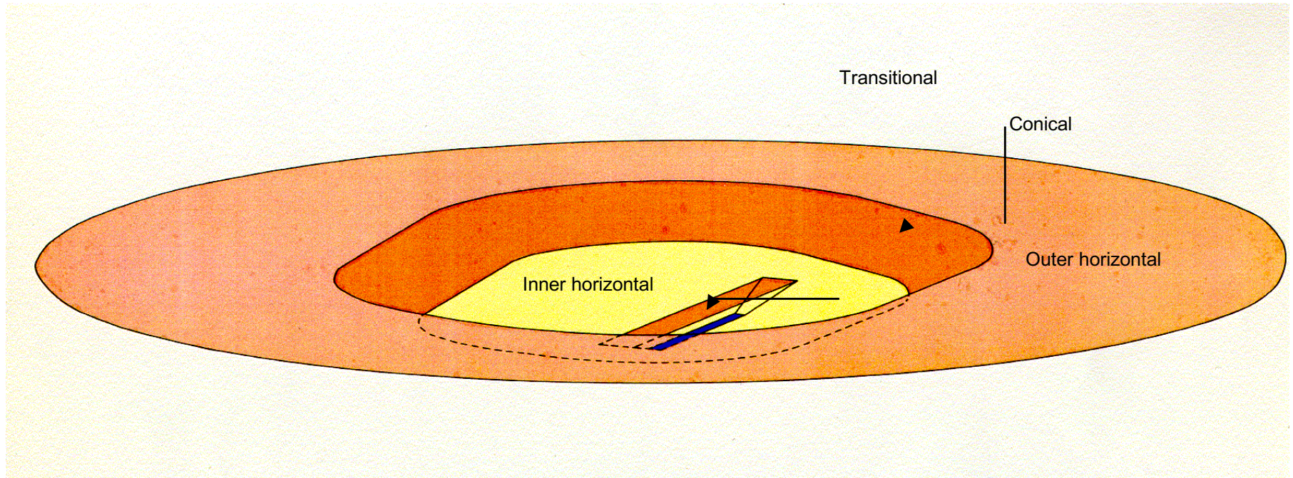
Figure 3-1: Relationship of outer horizontal, conical, inner horizontal and transitional surfaces
