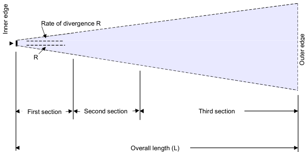
Figure 3-4: Plan view of approach surface
