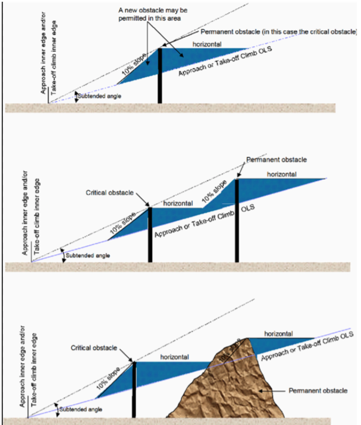
Figure 4-1: Shielding of obstacles penetrating the approach and take-off climb surface
