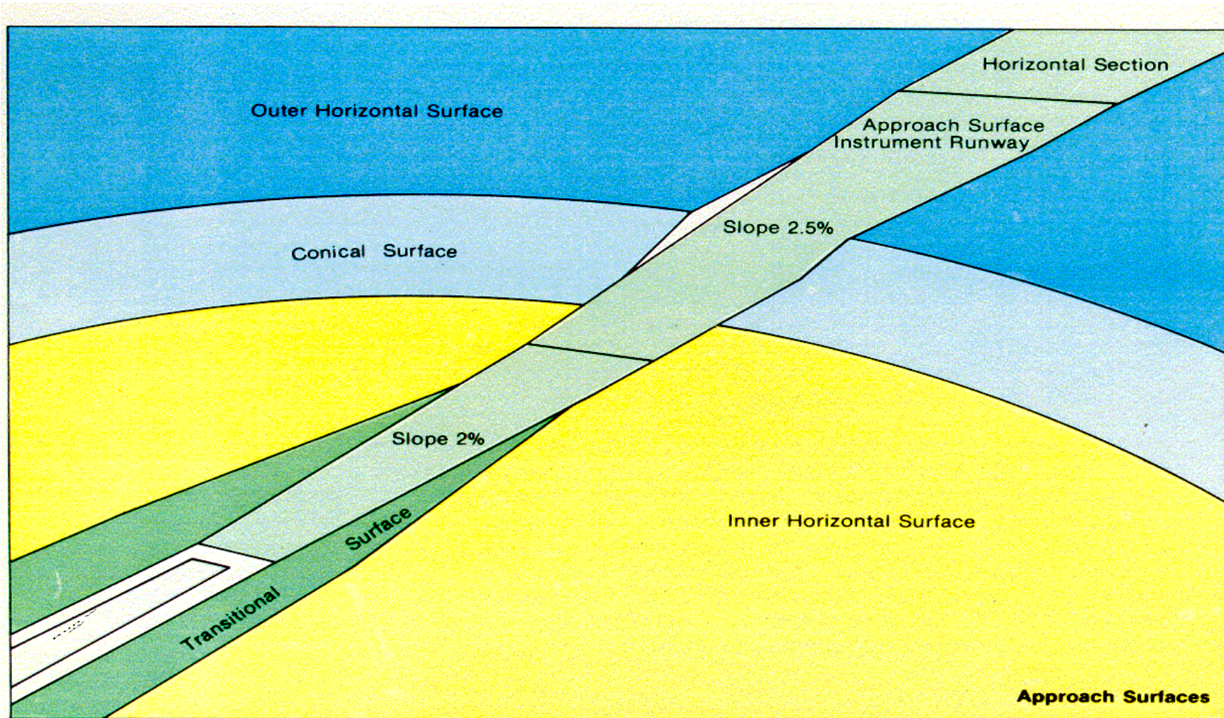
Figure.3-3: Approach surface for an instrument approach runway
