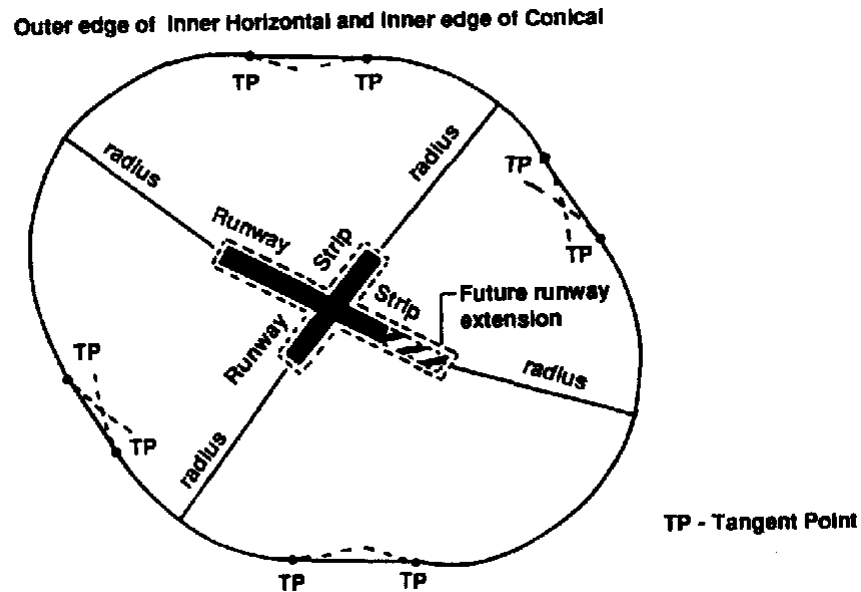
Figure 3-2: Boundary of inner horizontal surface
