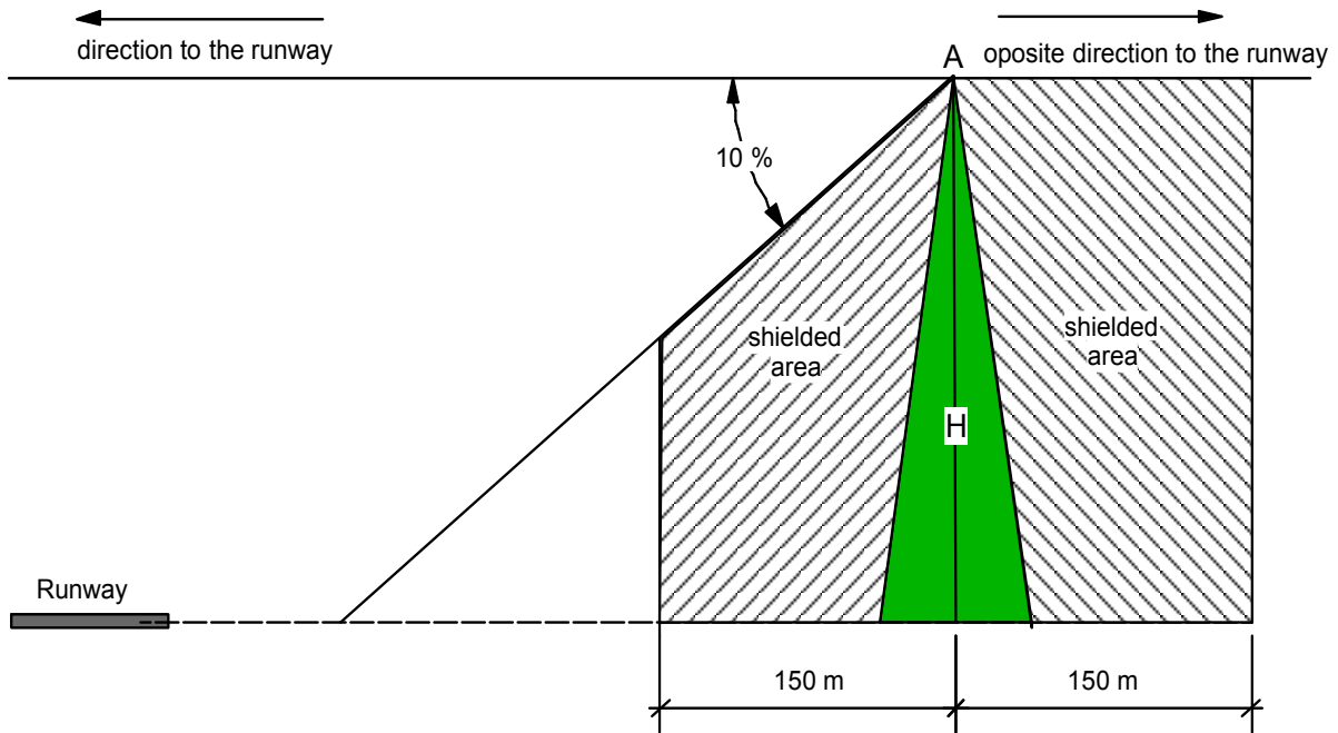
Fig. 4-2 Cross section of shielding principle
