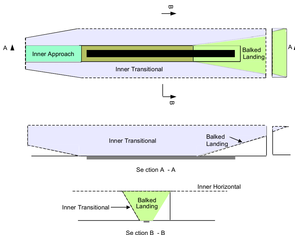
Figure 3-5: Inner approach, inner transitional and baulked landing obstacle limitation surfaces
