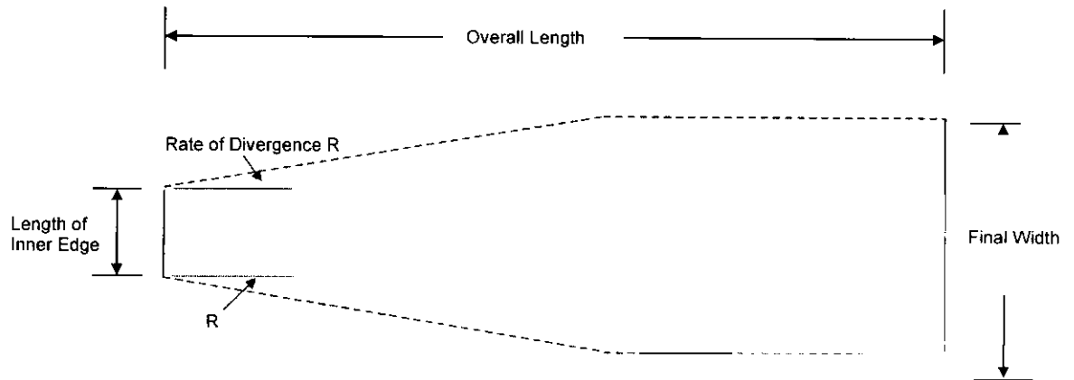
Figure 3-6: Plan view of take-off climb surface
