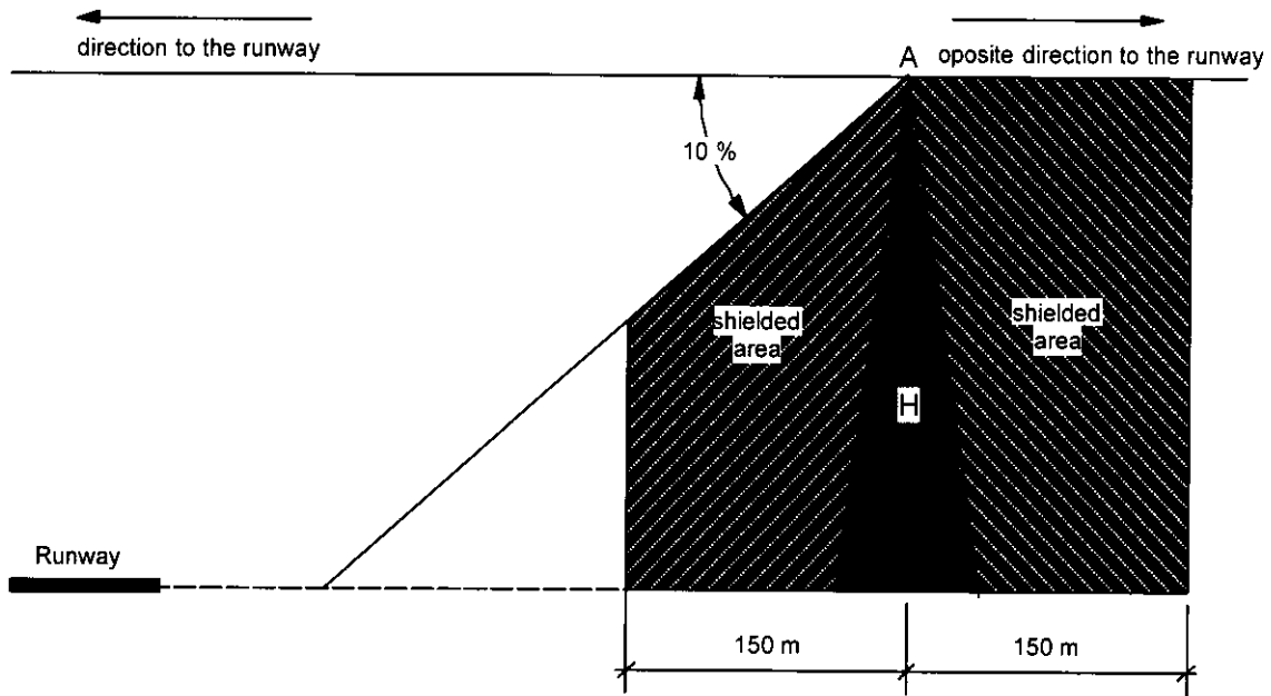
Fig. 4-2 Cross section of shielding principle
