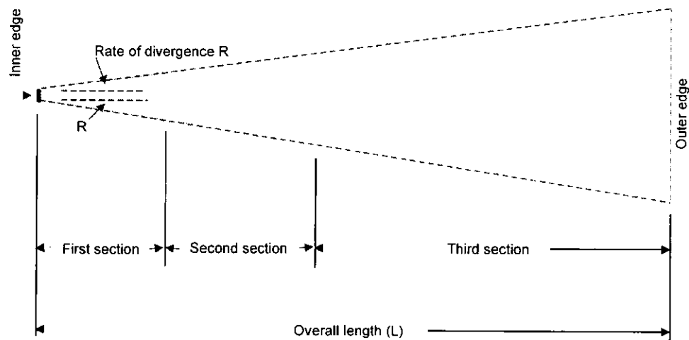
Figure 3-4: Plan view of approach surface
