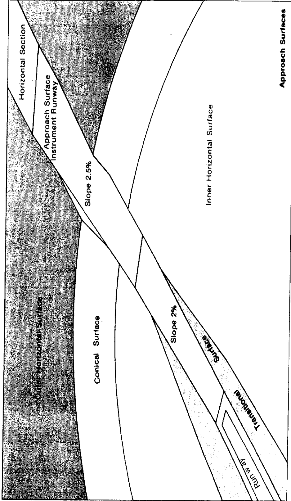
Figure.3-3: Approach surface for an instrument approach runway
